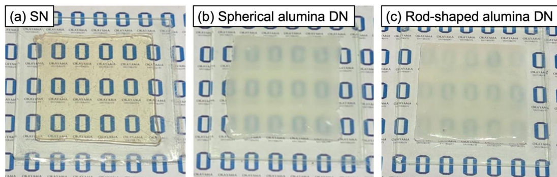
Figure 2 Photos of the PIL ion gels (a: SN, b: spherical alumina DN, c: rod-shaped alumina DN).
