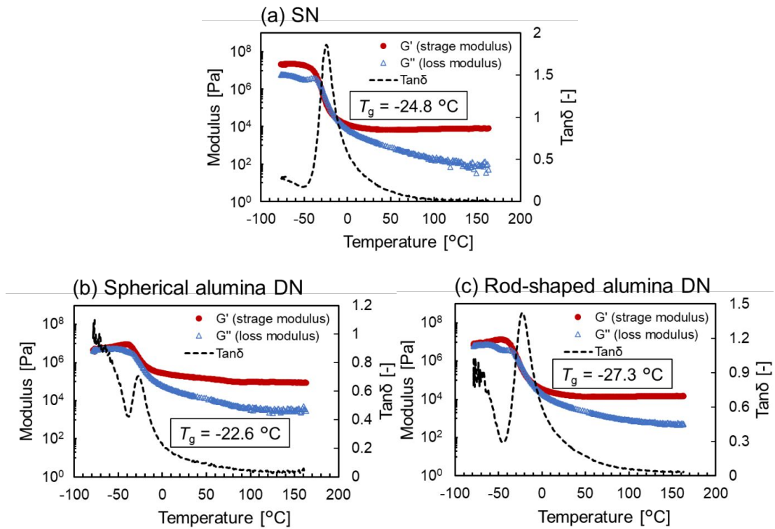
Figure S3 Oscillatory shear temperature-sweep viscoelasticity measurements of (a) PIL SN, (b) spherical alumina/PIL DN, and (c) rod-shaped alumina/PIL DN ion gels.
