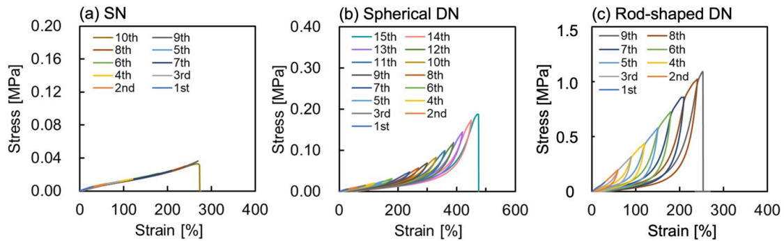
Figure 6 Cyclic tensile tests of (a) PIL SN, (b) spherical alumina/PIL DN, and (c) rod-shaped alumina/PIL DN ion gels.
