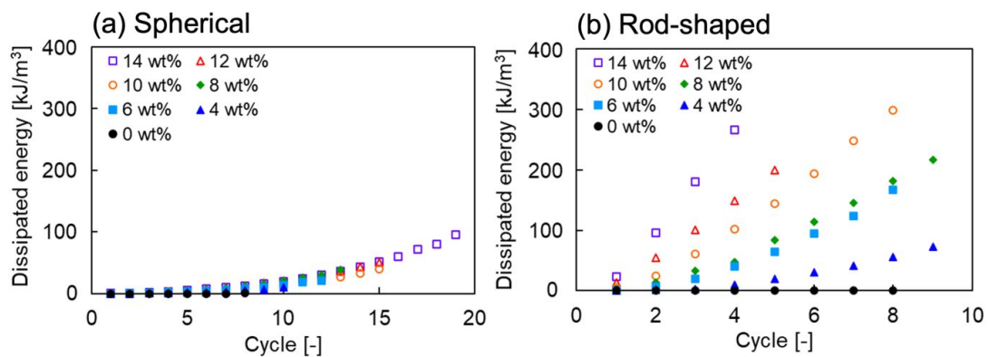
Figure 7 Dissipated energy of (a) spherical alumina/PIL DN and (b) rod-shaped alumina/PIL DN ion gels, as a function of cycle.
