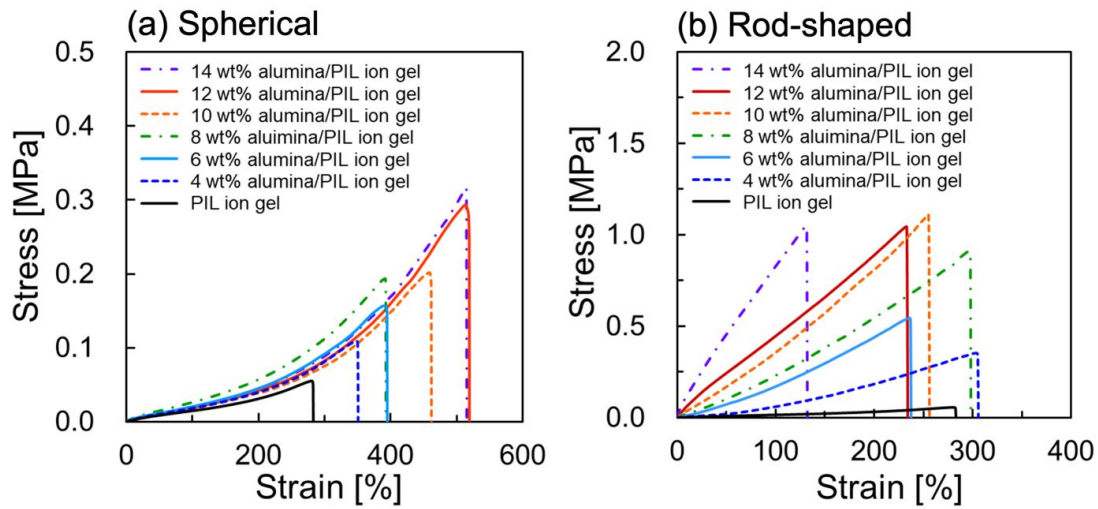
Figure 4 Stress–strain curves of (a) spherical and (b) rod-shaped alumina/PIL DN ion gels with different alumina concentrations.
