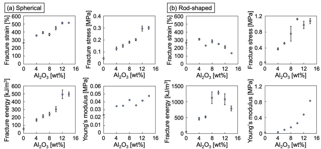
Figure 5 Mechanical properties of (a) spherical and (b) rod-shaped alumina/PIL DN ion gels with different alumina concentration.
