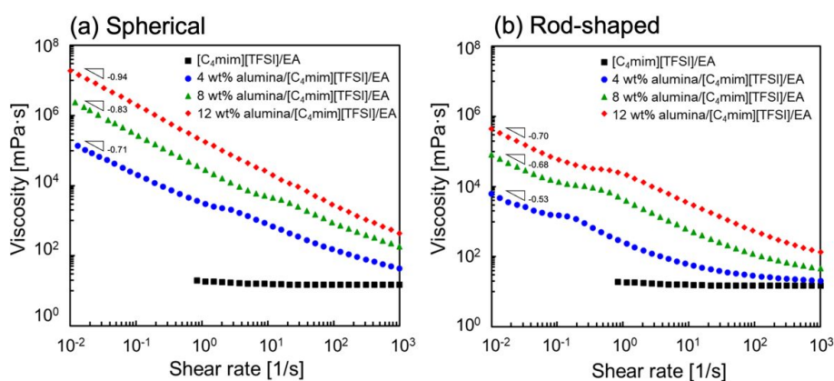
Figure 1 Shear rate dependencies on the viscosities of the IL dispersions of different concentrations of (a) spherical and (b) rod-shaped alumina.
