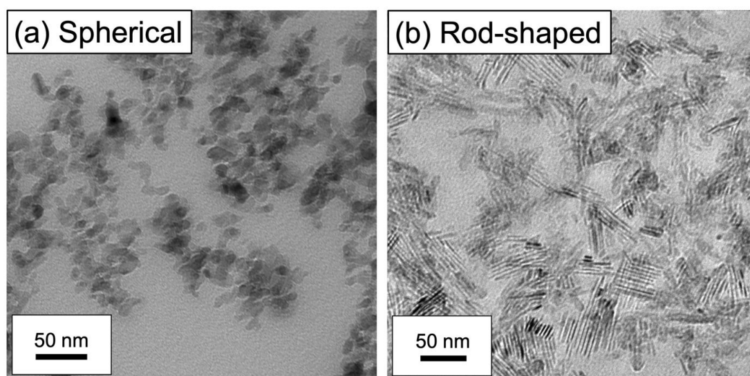
Figure 3 TEM images of the PIL ion gels with (a) spherical and (b) rod-shaped alumina.
