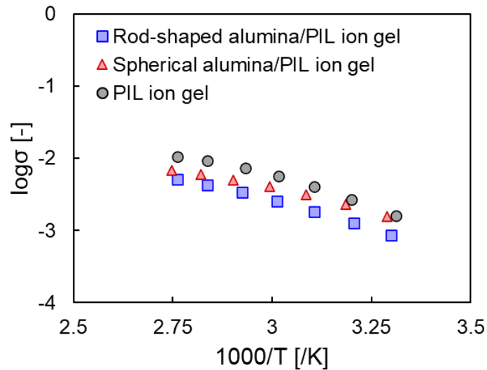
Figure S4 Ionic conductivity ( \sigma ) of PIL DN ion gels with different shapes of alumina and PIL SN ion gel.
